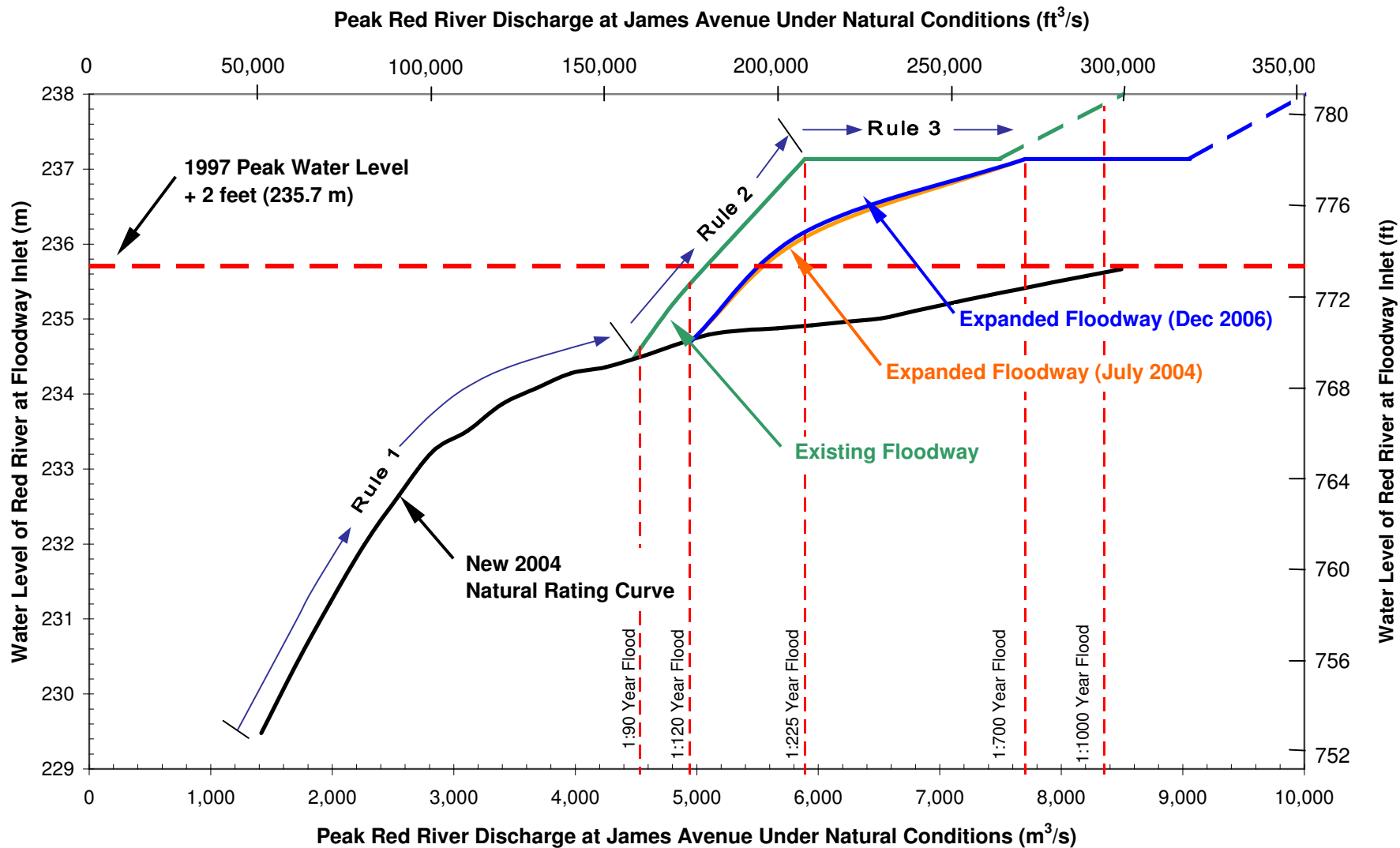
Figure 5.3-4 Application of Floodway Operation Rules for Expanded Floodway
