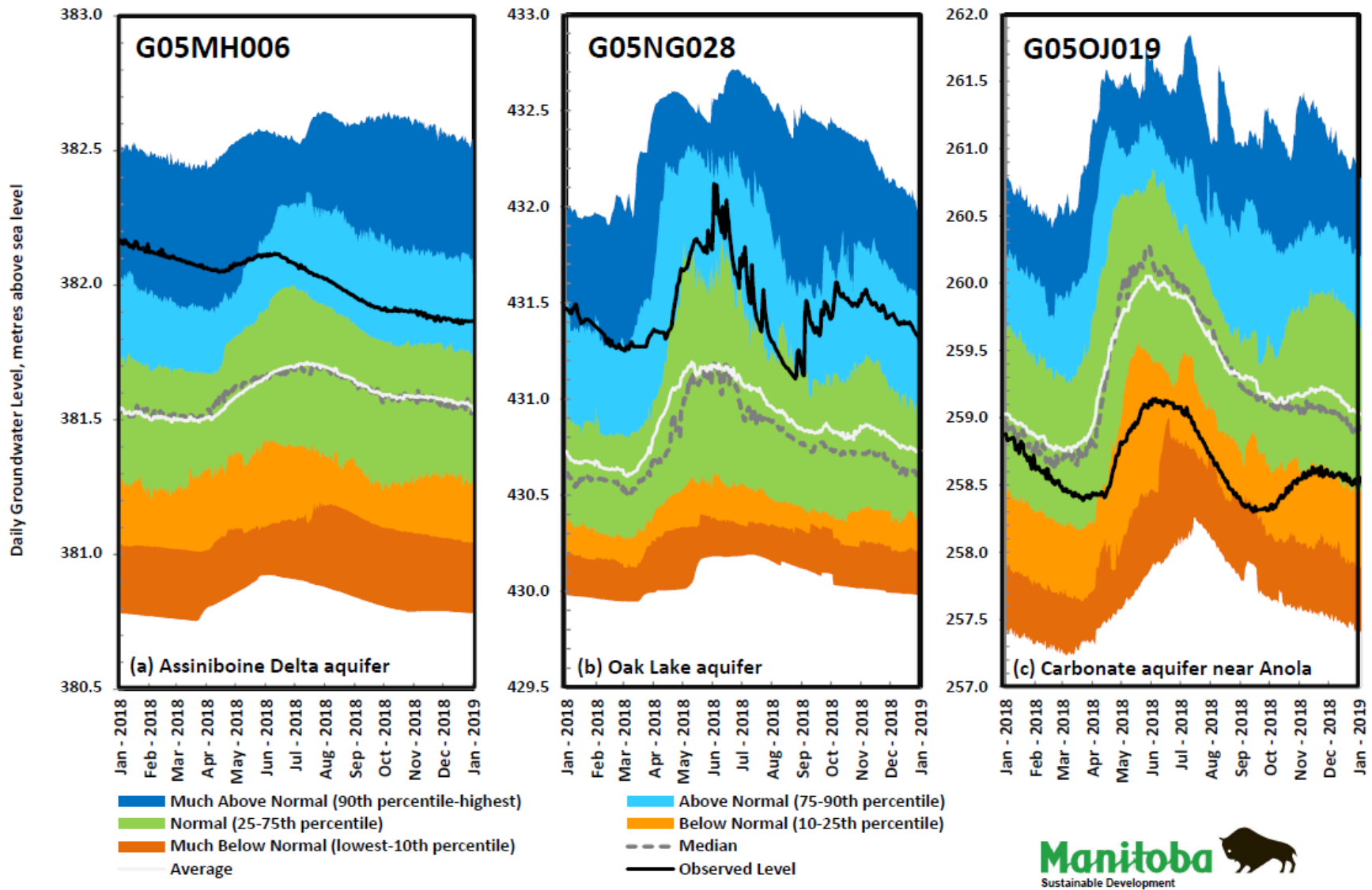
Figure 6: Groundwater hydrographs for (a) the Assiniboine Delta aquifer, (b) the Oak Lake aquifer, and (c) the Carbonate aquifer near Anola for 2018. Data provided by the Groundwater Management Section of Manitoba Sustainable Development.
