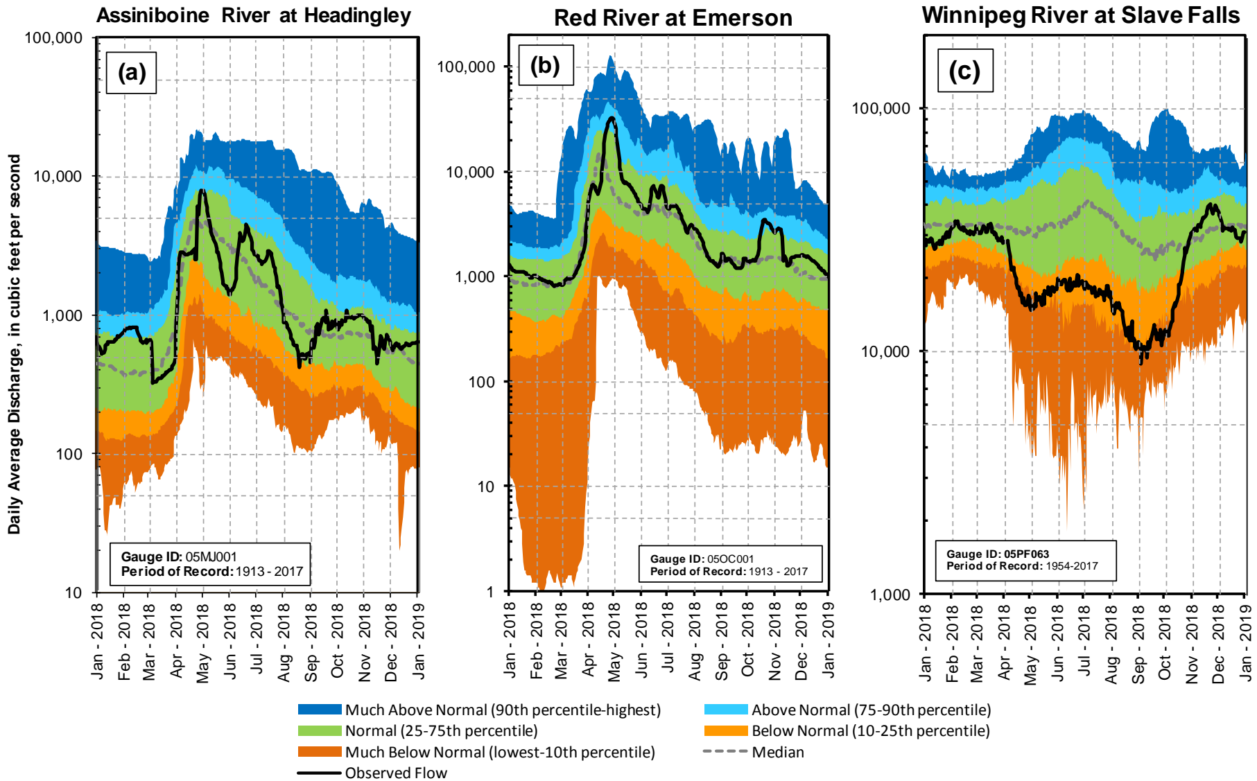
Figure 4: Daily streamflow percentile plots for the (a) Assiniboine, (b) Red, and (c) Winnipeg Rivers for 2018. Hydrometric data are obtained from Water Survey of Canada and Manitoba Hydro. Near real-time data are preliminary and subject to change upon review. All of the above gauges are classified as regulated.
