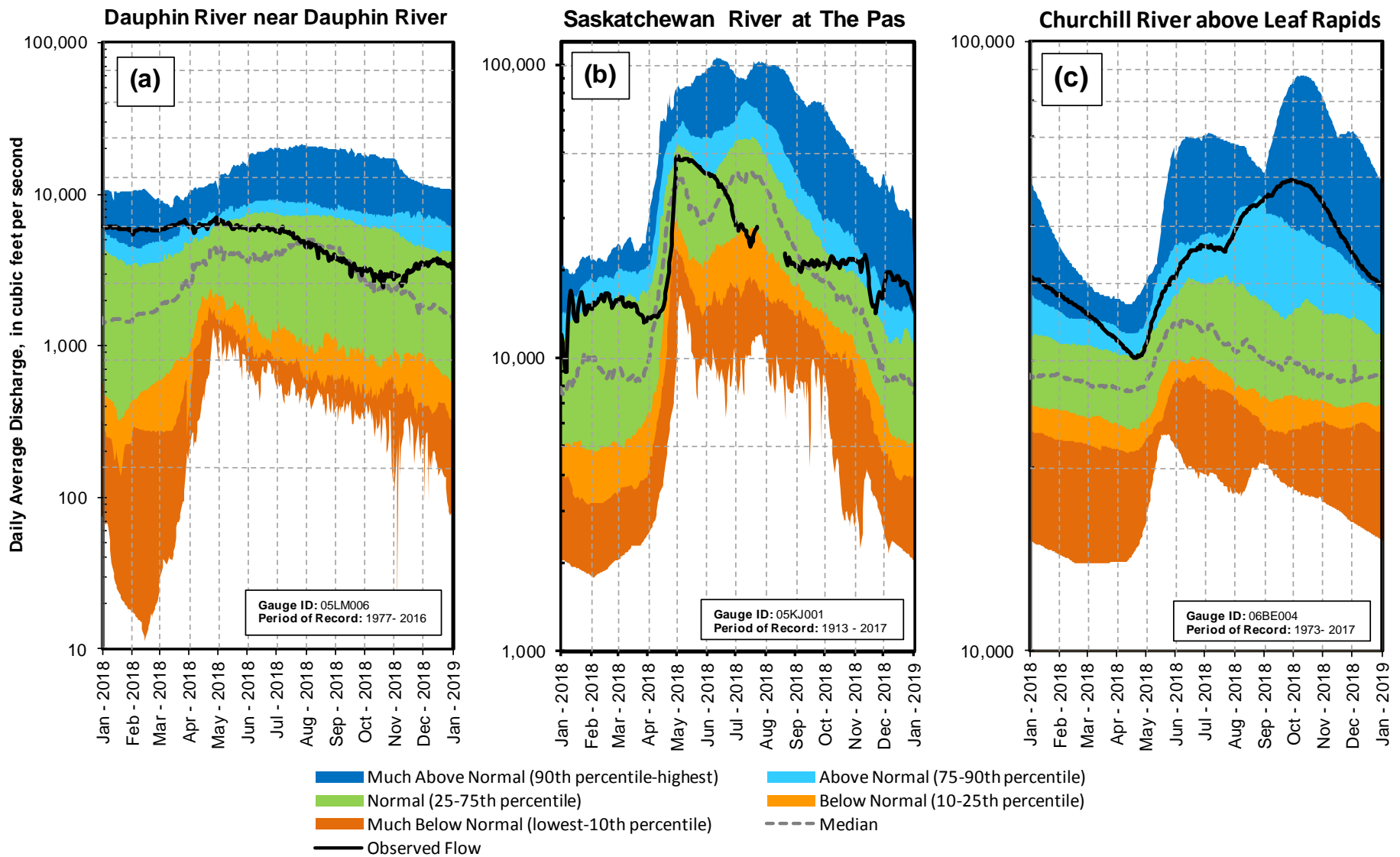
Figure 5: Daily streamflow percentile plots for the (a) Dauphin, (b) Saskatchewan, and (c) Churchill Rivers for 2018. Hydrometric data are obtained from Water Survey of Canada. Near real-time data are preliminary and subject to change upon review. All of the above gauges are classified as regulated.
